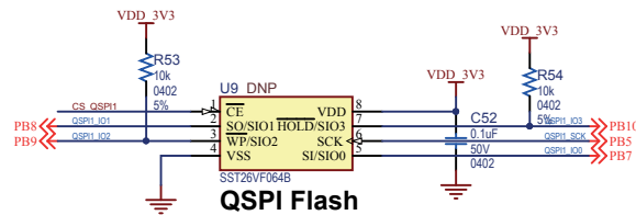
Figure 3-12. Optional QSPI Serial Data Flash on Baseboard
