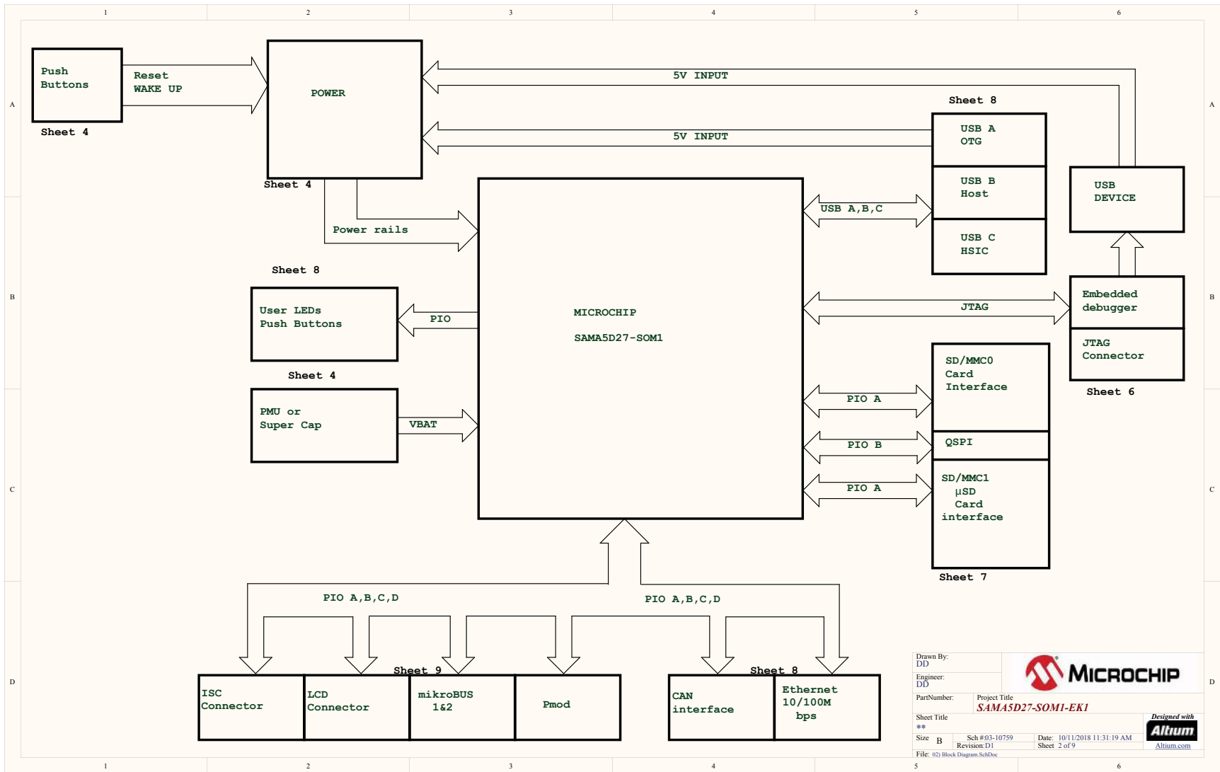
Figure 6-2. Block Diagram
