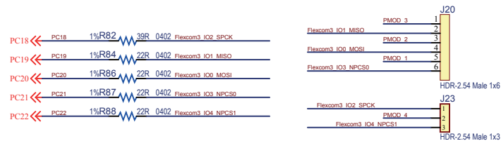
Figure 3-49. Pmod Jumper Configuration
