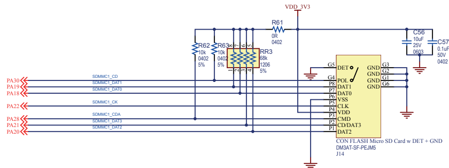
Figure 3-16. SDMMC1 microSD
