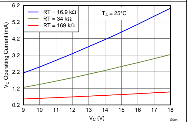
Figure 8. VC Operating Current vs VC Voltage
