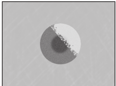
Oblique Illumination—UNACCEPTABLE
