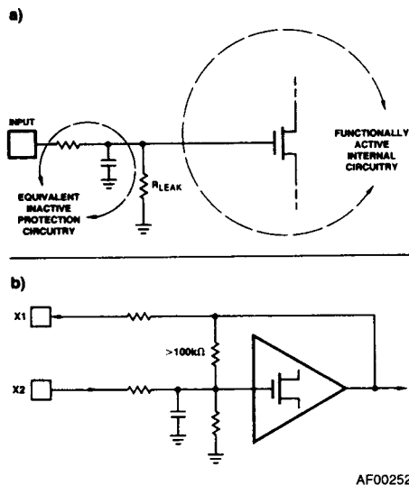
Figure 3. Input Circuitry
