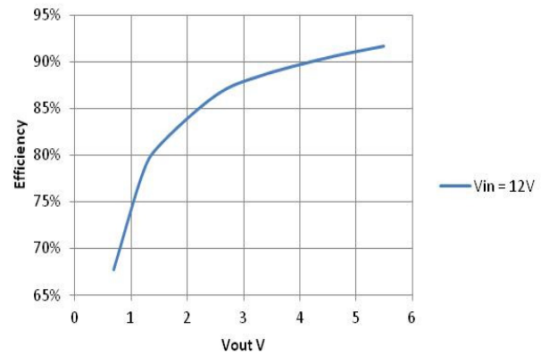
Figure 5. Efficiency vs. Output Voltage, I_{out}=7\text{A} , F_{sw}=500\text{kHz}
