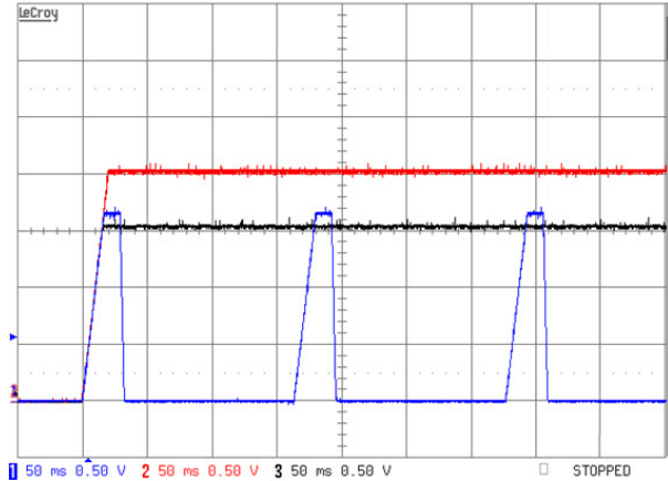
Figure 33. Turn-On into UVP on V3. The UV Fault Is Programmed To Be Non-Latching. Ch1 – Vo1, Ch2 – Vo2(Group A), Ch3 – Vo3 (Group B) Vo4 not shown.
