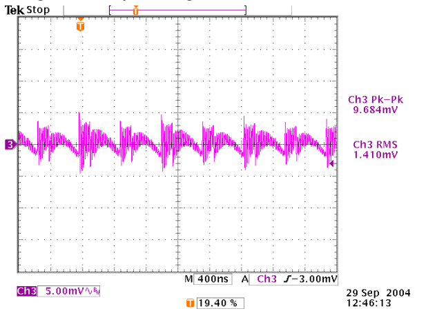
Figure 42. Output Voltage Noise, Full Load, 180° Interleave
