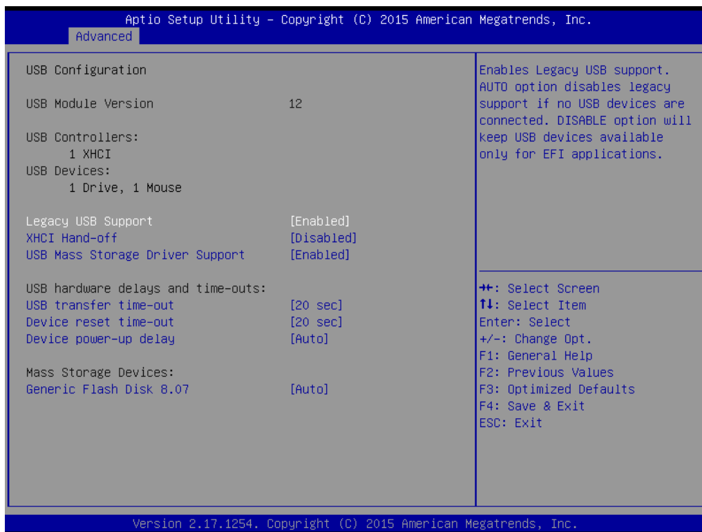
Figure 3.20 USB Configuration
