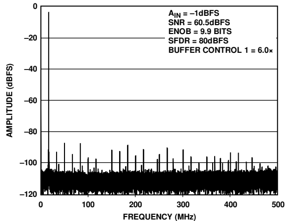
Figure 11. Single-Tone FFT with f_{IN} = 985.3 MHz
