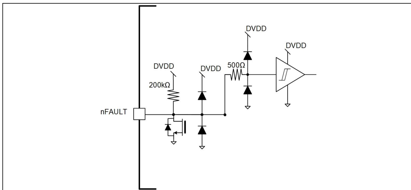
Figure 68 ESD protection and pin diagram for nFAULT open drain pin
