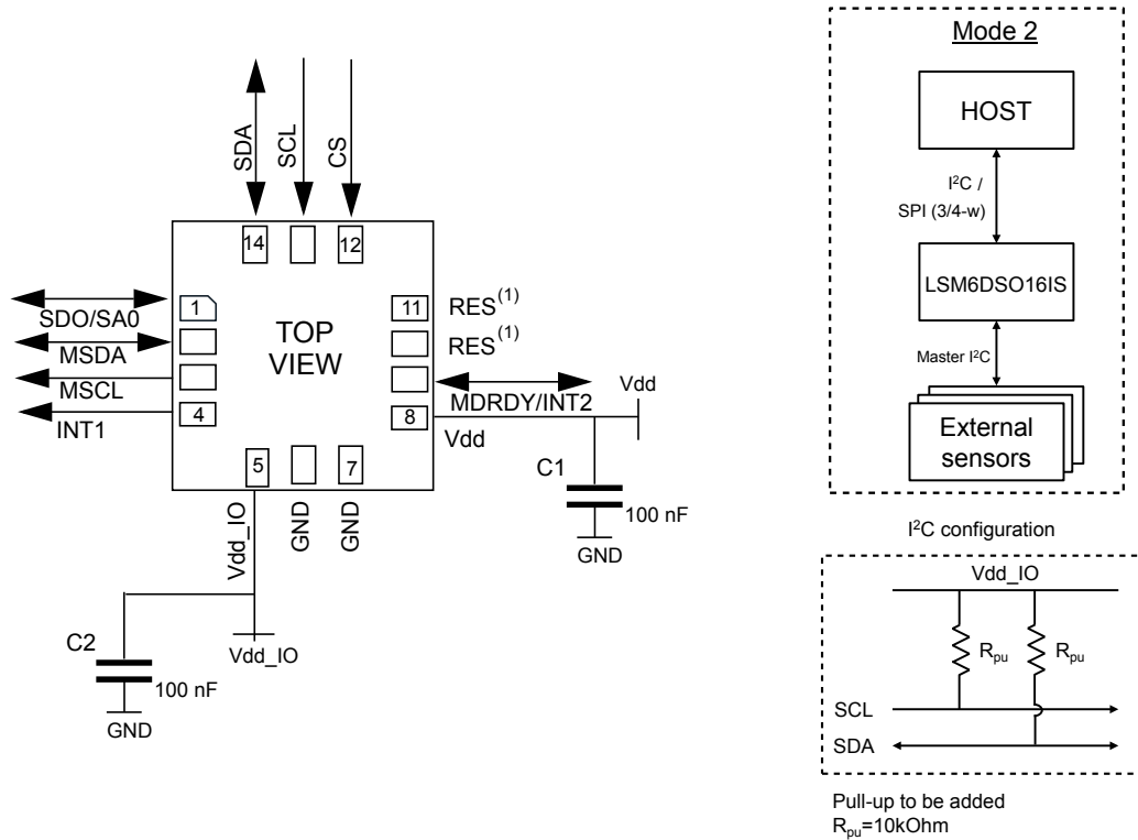
Figure 16. LSM6DSO16IS electrical connections in mode 2
