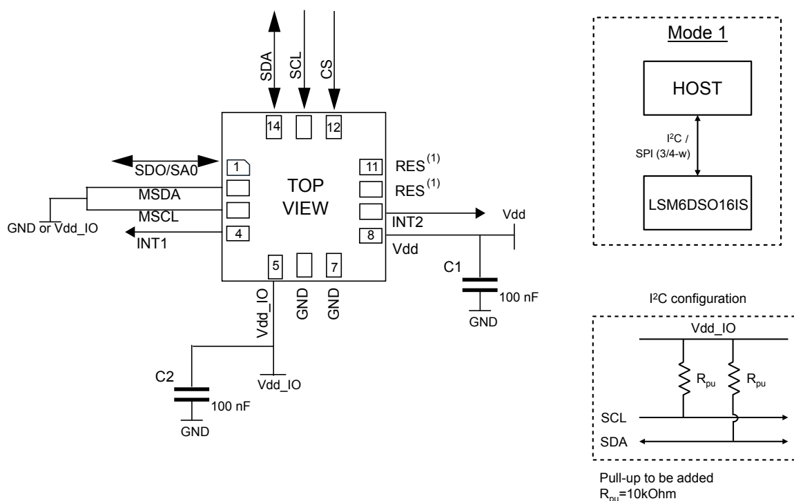
Figure 15. LSM6DSO16IS electrical connections in mode 1
