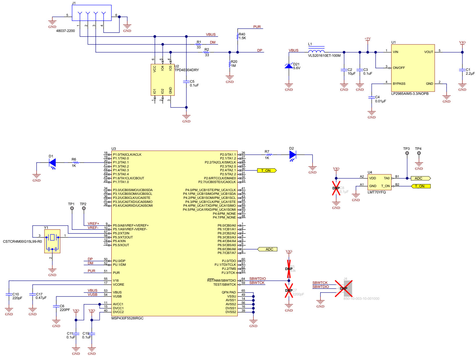
Figure 7-1. LMT70EVM Schematic
