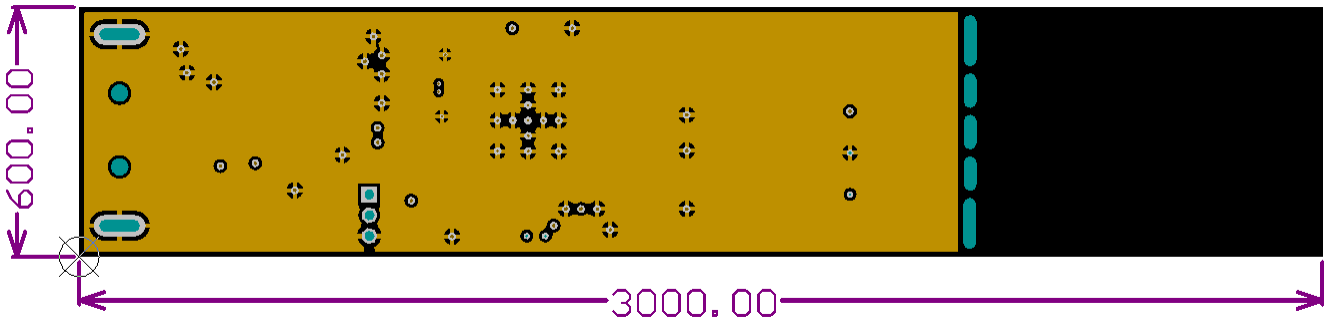
Figure 6-4. Ground Layer Routing
