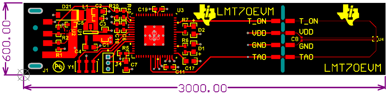
Figure 6-1. Top Assembly Layer
