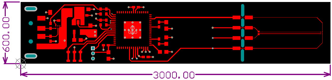
Figure 6-2. Top Layer Routing
