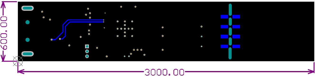
Figure 6-5. Bottom Layer Routing
