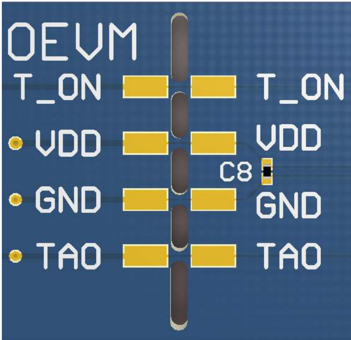
Figure 4-6. Breakout Slots and Exposed Pads
