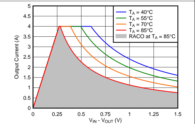
Figure 62. Recommended Area for Continuous Operation for V_{OUT} = 2.5\text{ V}
