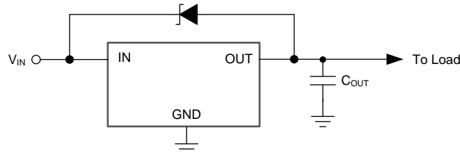
Figure 55. Zener Diode Placed from IN to OUT
