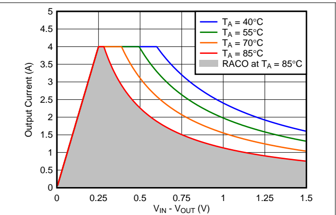
Figure 60. Recommended Area for Continuous Operation for V_{OUT} = 1.2\text{ V} with Bias
