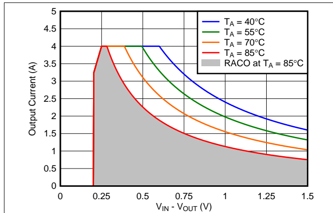
Figure 59. Recommended Area for Continuous Operation for V_{OUT} = 0.9\text{ V} with Bias
