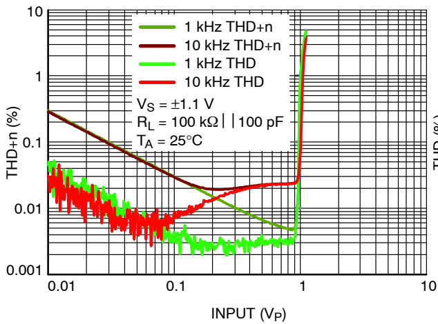
Figure 23. Harmonic Distortion
