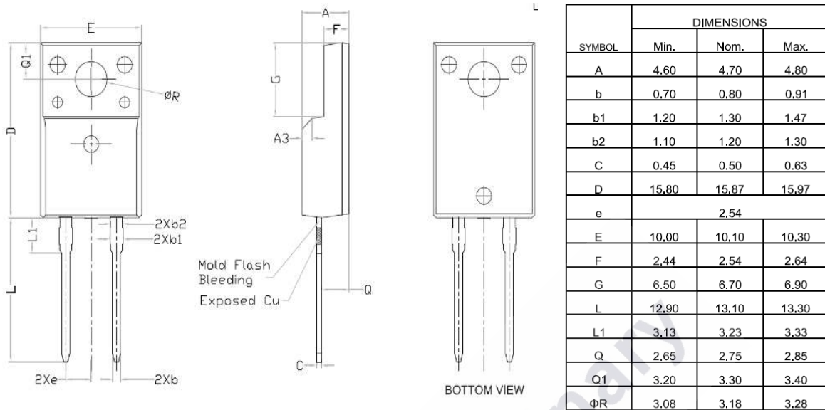
Drawing and dimensions
