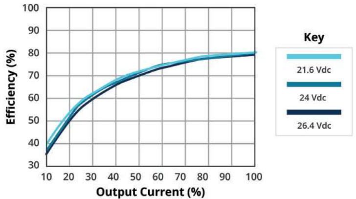
EFFICIENCY VS OUTPUT LOAD PCSA1-S24-12-S
