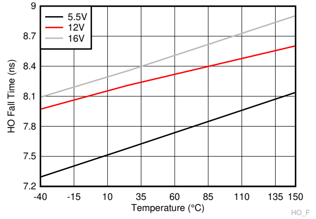
A. C_L=1800pF Figure 6-20. HO Fall Time
