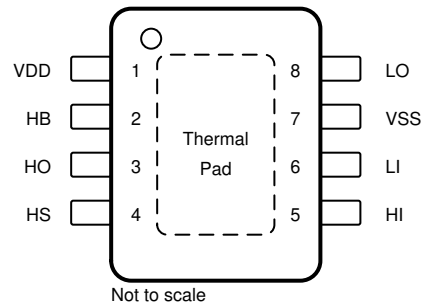
Figure 5-2. DDA Package 8-Pin SOIC with PowerPAD Top View
