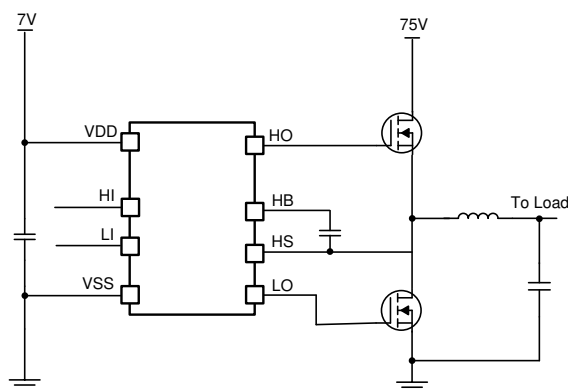
Simplified Application Diagram
