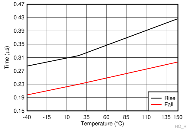
A. C_L=100nF Figure 6-22. HO Rise andamp; Fall Time
