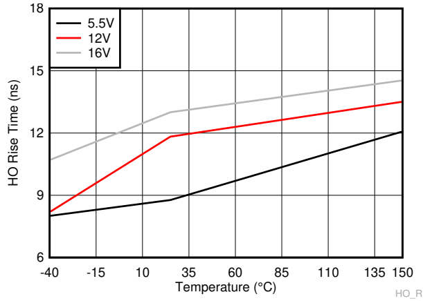
A. C_L=1800pF Figure 6-19. HO Rise Time
