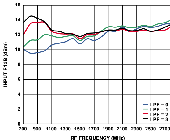
Figure 51. Input P1dB vs. RF Frequency for All LPF Settings, RFB and VGS Use Optimum Settings
