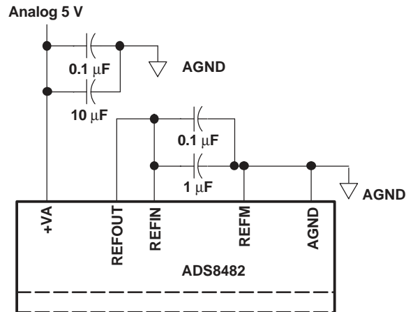
Figure 36. ADS8482 Using Internal Reference
