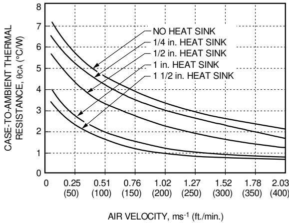
Figure 20. Case-to-Ambient Thermal Resistance Curves; Either Orientation
