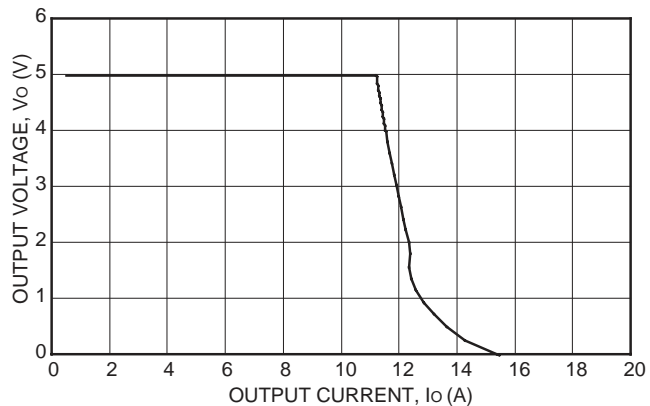
Figure 2. Typical Output Characteristics at Room Temperature
