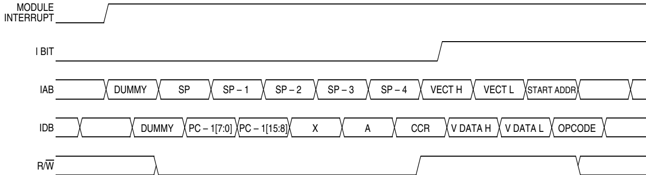
Figure 5-9. Interrupt Entry
