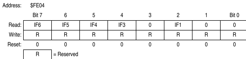
Figure 5-12. Interrupt Status Register 1 (INT1)
