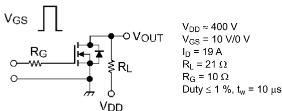
Fig. 6.2.1 Switching Time Test Circuit
