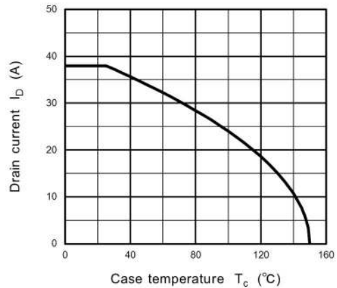
Fig. 8.17 I_D - T_c (Guaranteed Maximum)
