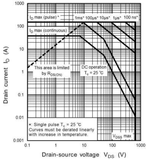
Fig. 8.18 Safe Operating Area (Guaranteed Maximum)
