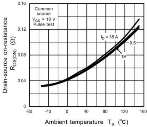
Fig. 8.7 R_{DS(ON)} - T_a
