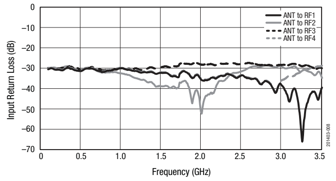
Figure 8. Input Return Loss vs Frequency
