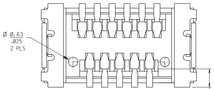
BOTTOM VIEW OF CONNECTOR
