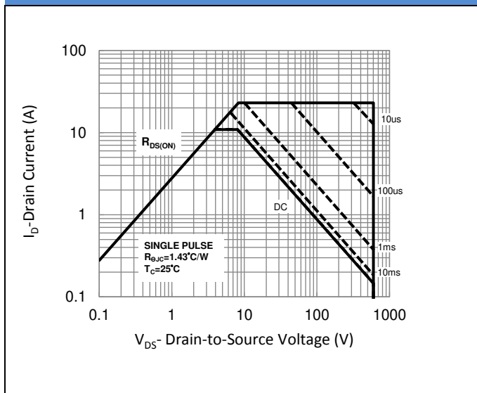
Fig.11 Maximum Safe Operating Area
