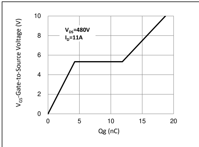
Fig.7 Gate-Charge Characteristics
