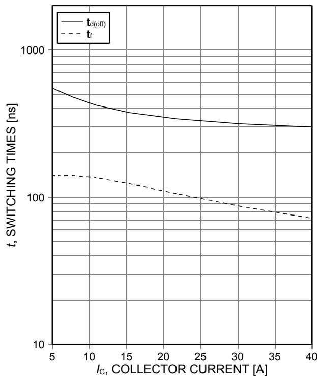
Figure 8. Typical switching times as a function of collector current (inductive load, T_{vj}=175^\circ\text{C} , V_{CE}=600\text{V} , V_{GE}=0/15\text{V} , R_{G(on)}=10\Omega , R_{G(off)}=10\Omega , dynamic test circuit in Figure E)
