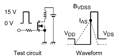
Fig. 9.15 Test Circuit/Waveform
