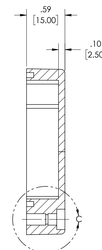
SECTION B-B SCALE 1 : 0.75
