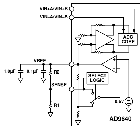
Figure 52. Programmable Reference Configuration
