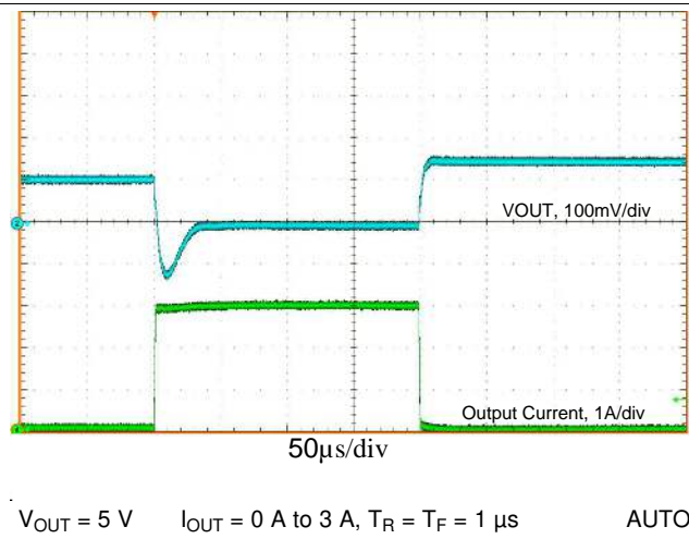
Figure 30. Load Transients
