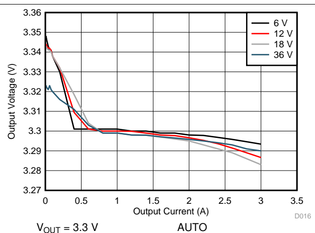
Figure 34. Load and Line Regulation
