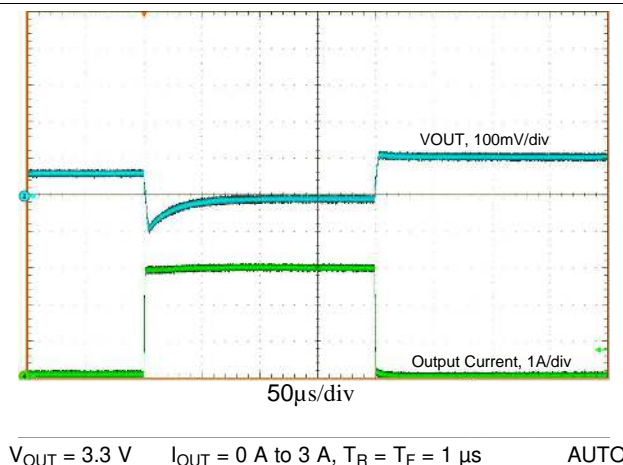
Figure 42. Load Transient
