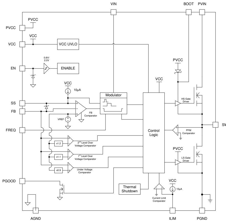
Figure 2. Block Diagram
