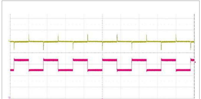
Output voltage response to load current step-change (1.85-2.77-1.85 A) at: T_{P1} = +25^{\circ}\text{C} , V_i = 110\text{ V} . Top trace: output voltage (500 mV/div.). Bottom trace: load current (1 A/div.). Time scale: (2 ms/div.).
