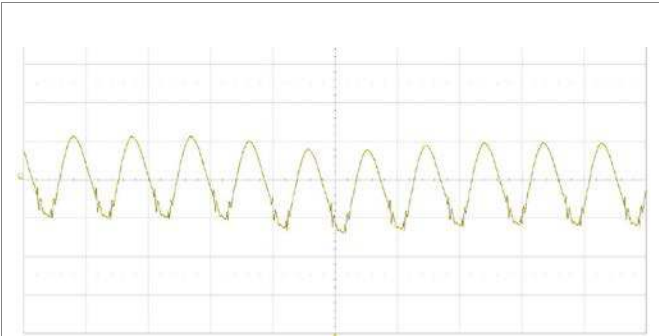
Output voltage ripple at: T_{P1} = +25^{\circ}\text{C} , V_i = 110\text{ V} , I_o = 3.7\text{ A} resistive load. Trace: output voltage (20 mV/div.). Time scale: (5 μs/div.). 20 MHz bandwidth
