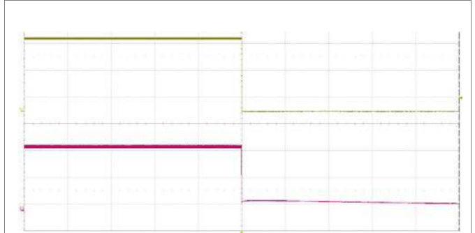
Shut-down enabled by disconnecting V_i at: T_{P1} = +25^{\circ}\text{C} , V_i = 110\text{ V} , I_o = 3.7\text{ A} resistive load. Top trace: output voltage (20 V/div.). Bottom trace: input voltage (50 V/div.). Time scale: (200 ms/div.).
