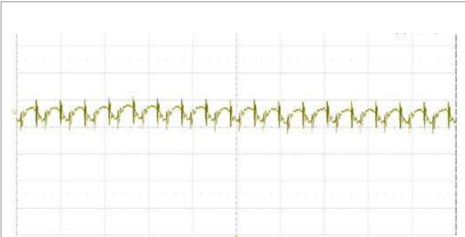
Output voltage ripple at: T_{P1} = +25^\circ\text{C} , V_i = 110\text{ V} , I_o = 8.33\text{ A} resistive load. Trace: output voltage (20 mV/div.). Time scale: (5 μs/div.). 20 MHz bandwidth
