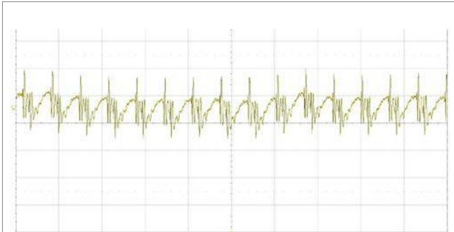
Output voltage ripple at: T_{P1} = +25^\circ\text{C} , V_I = 110\text{ V} , I_O = 16.67\text{ A} resistive load. Trace: output voltage (20 mV/div.). Time scale: (5 μs/div.). 20MHz bandwidth
