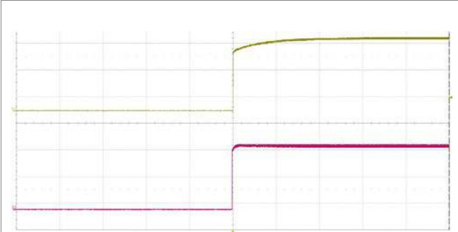
Start-up enabled by connecting V_i at: T_{P1} = +25^{\circ}\text{C} , V_i = 110\text{ V} , I_o = 3.7\text{ A} resistive load. Top trace: output voltage (20 V/div.). Bottom trace: input voltage (50 V/div.). Time scale: (200 ms/div.).
