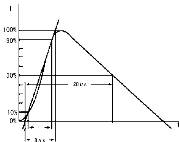
Fig. 10.2 Based on IEC61000-4-5 8/20 \mu s pulse. (Ed.2)
