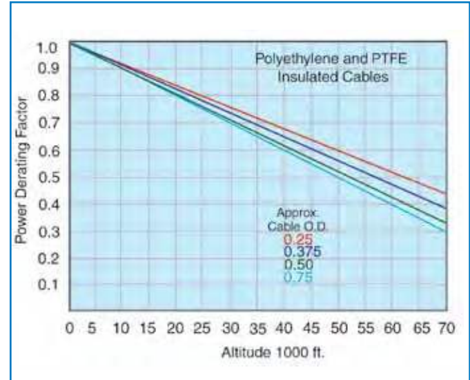
Fig. 7 Power Altitude Correction Factor
