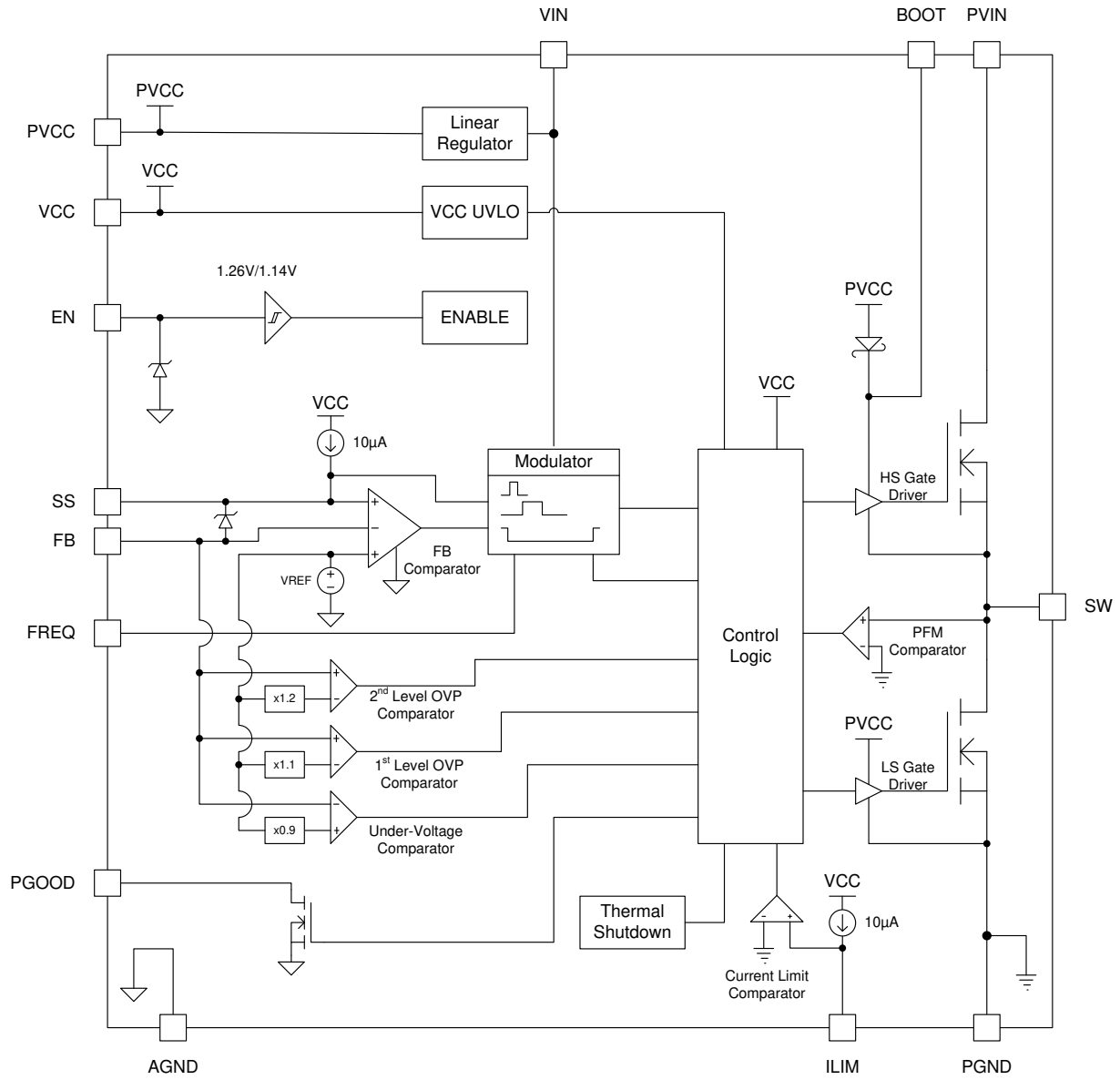
Figure 3. Block Diagram
