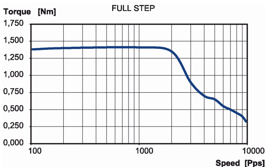
Figure 4.2: QSH6018-56-28-165 Speed vs. Torque Characteristics
