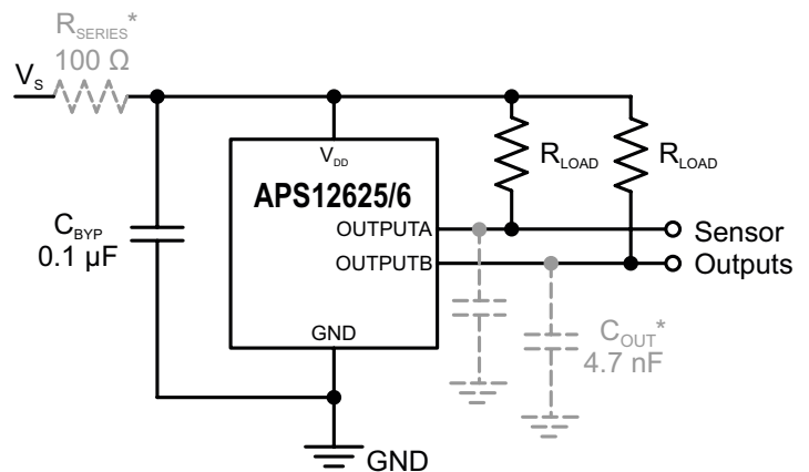
Figure 13: Typical Application Circuit
