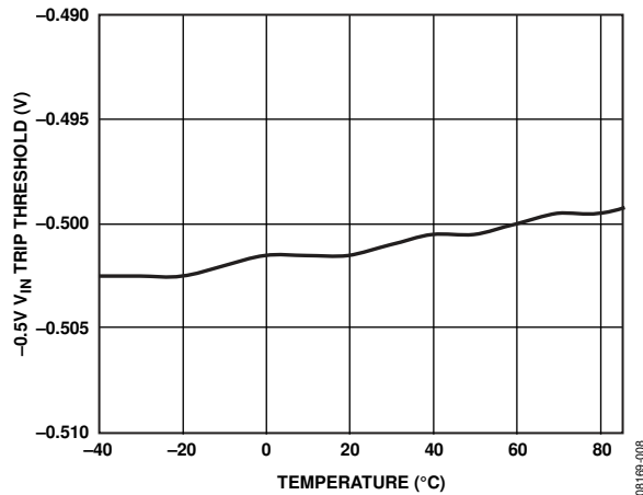
Figure 12. -0.5 V Input Voltage Trip Threshold vs. Temperature
