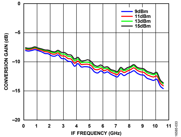
Figure 33. Conversion Gain vs. IF Frequency at Various LO Drives, LO Frequency = 18 GHz
