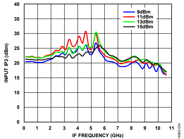
Figure 34. Input IP3 vs. IF Frequency at Various LO Drives, LO Frequency = 18 GHz
