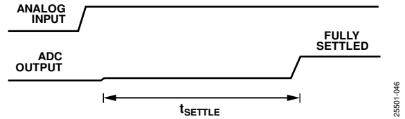
Figure 48. Step Input with Single Cycle Settling
