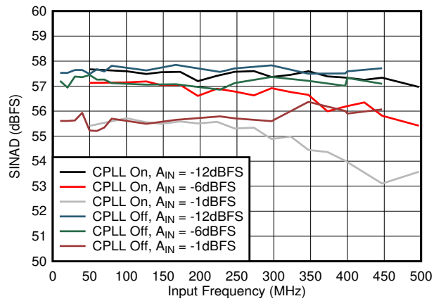
Figure 7-56. SINAD vs A_{IN} and C-PLL
