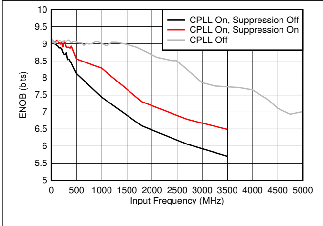
Figure 7-43. ENOB vs F_{IN} and C-PLL modes
