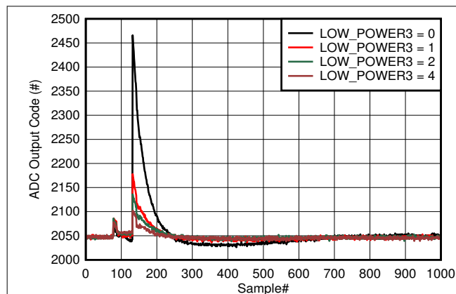
Figure 8-10. Background Calibration Core Transition In Low Power Mode
