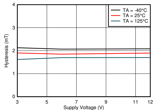
Figure 7-6. Hysteresis vs V CC
