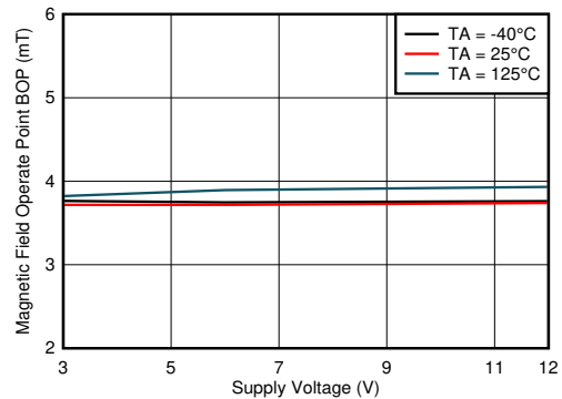
Figure 7-2. B OP vs V CC
