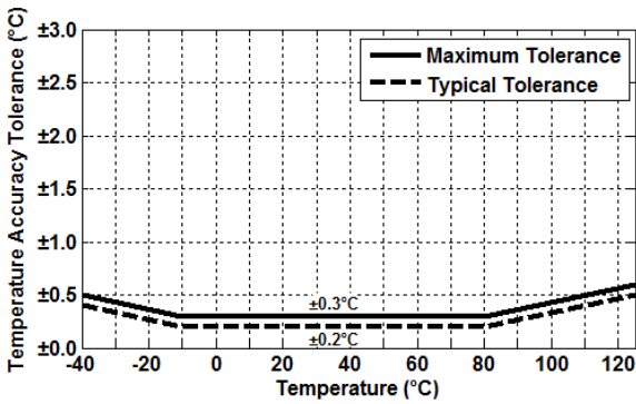
Figure 8. HS3101/HS3102 Temperature Sensor Accuracy Tolerance
