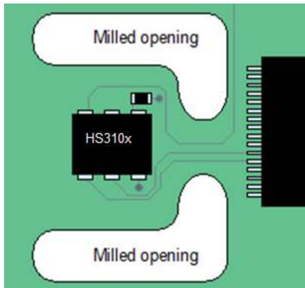
Figure 17. Milled PCB Openings for Thermal Isolation
