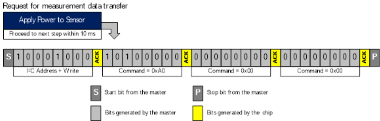
Figure 14. Sequence of Commands to Enter Programming Mode
