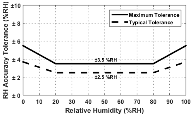
Figure 6. HS3103 RH Accuracy Tolerance at 25°C
