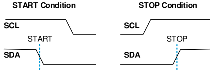
Figure 11. START and STOP Condition Waveform
