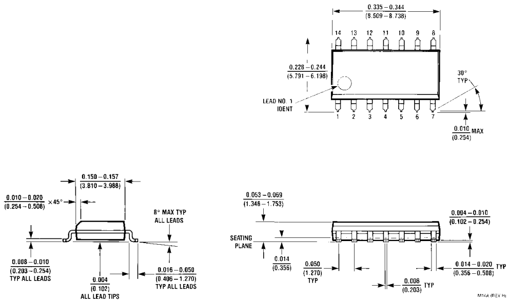
14-Lead Small Outline Molded Package (M) Order Number DM74LS05M NS Package Number M14A
