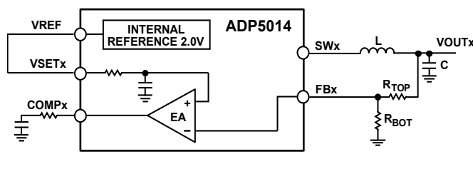
Figure 39. Configure the Output Voltage when V_{OUTx} > V_{REF}
