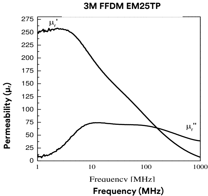
Figure 1. Real and Imaginary Part of Permeability with Frequency
