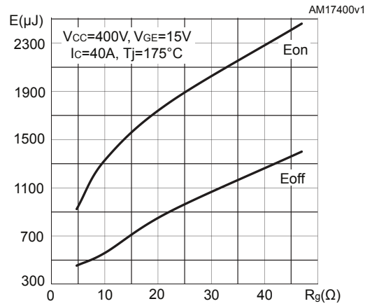
Figure 20. Switching energy vs gate resistance
