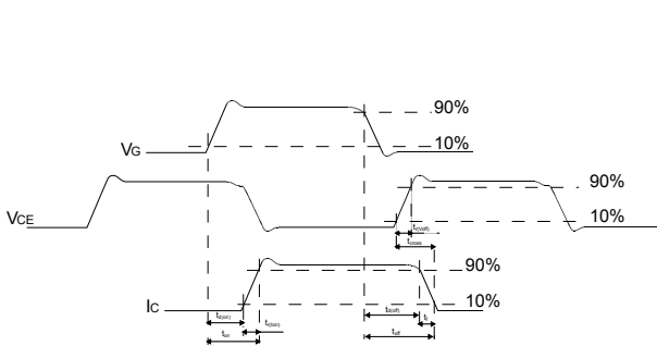
Figure 35. Switching waveform
