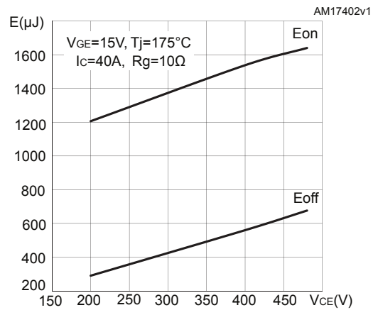
Figure 22. Switching energy vs collector emitter voltage
