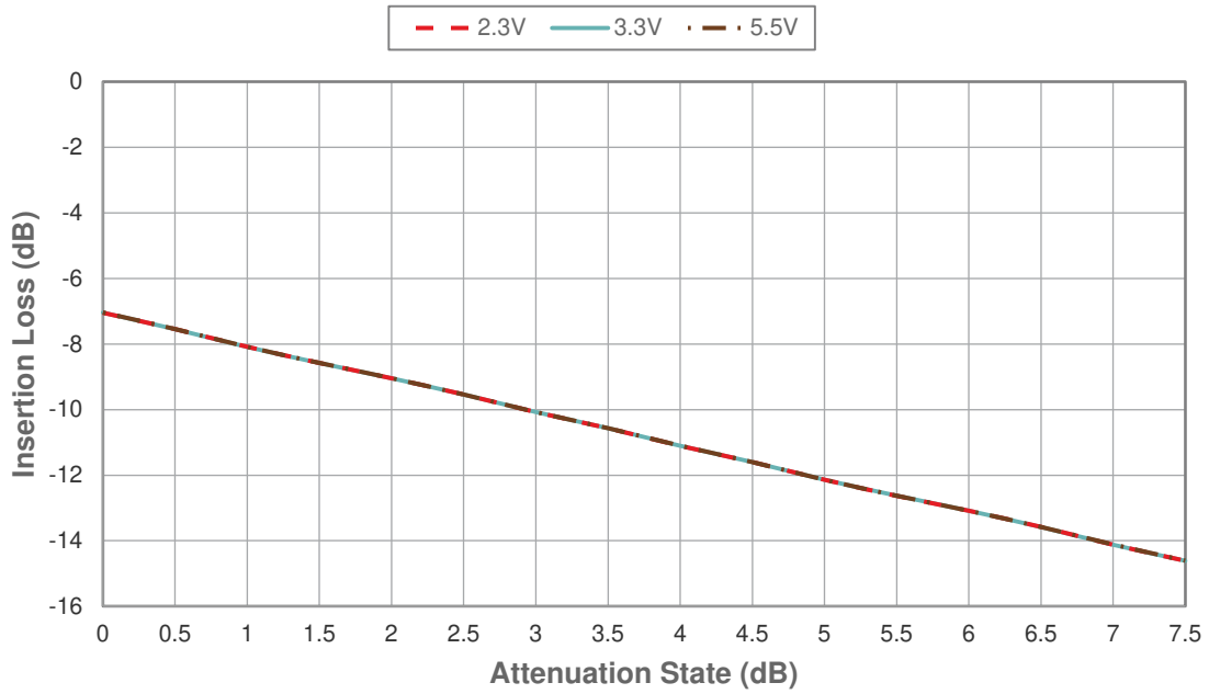
Figure 18 • RF_{OUT2} Insertion Loss Across RF_{OUT2} Attenuation State vs V_{DD} Frequency = 2.5 GHz
