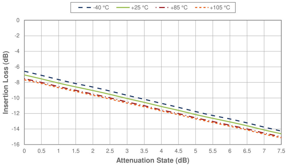
Figure 19 • RF_{OUT2} Insertion Loss Across RF_{OUT2} Attenuation State vs Temperature, Frequency = 2.5 GHz
