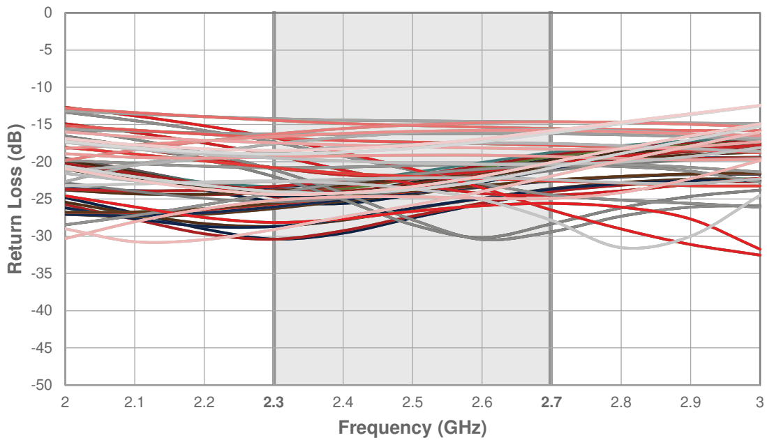
Figure 11 • Output Return Loss RF_{OUT2} (All RF_{OUT2} Phase States)
