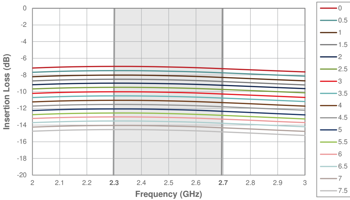
Figure 6 • Insertion Loss RF_{IN} - RF_{OUT2} (All RF_{OUT2} Attenuation States)
