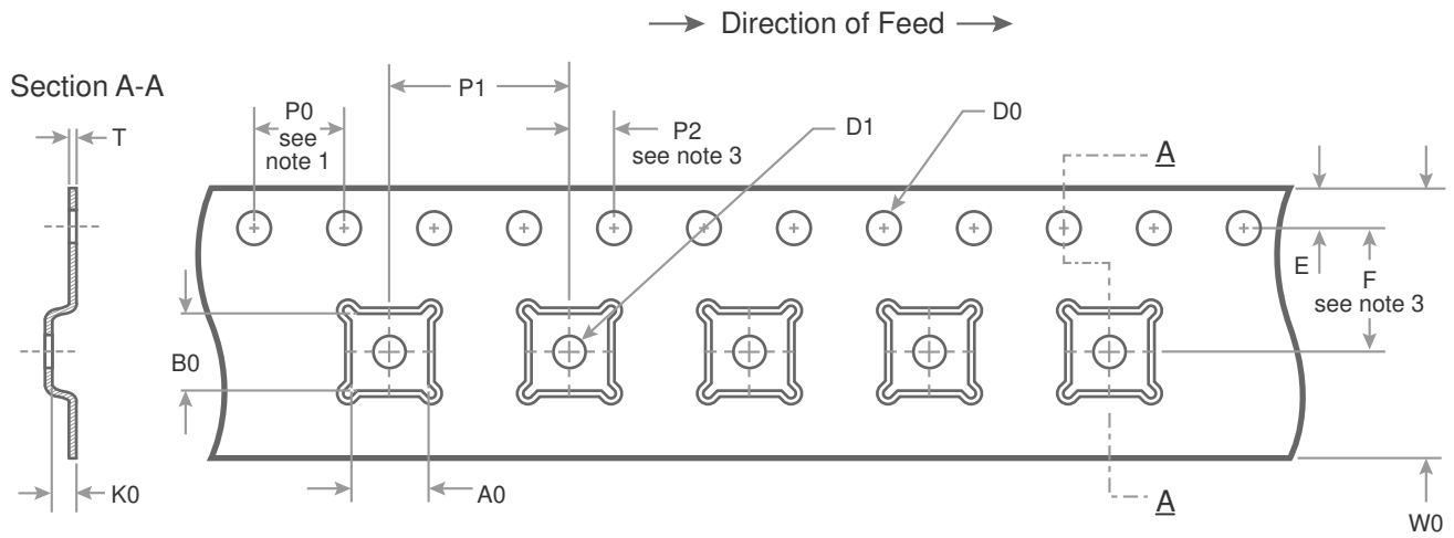
Figure 25 • Tape and Reel Specifications for 32-lead 6 × 6 × 0.85 mm QFN
