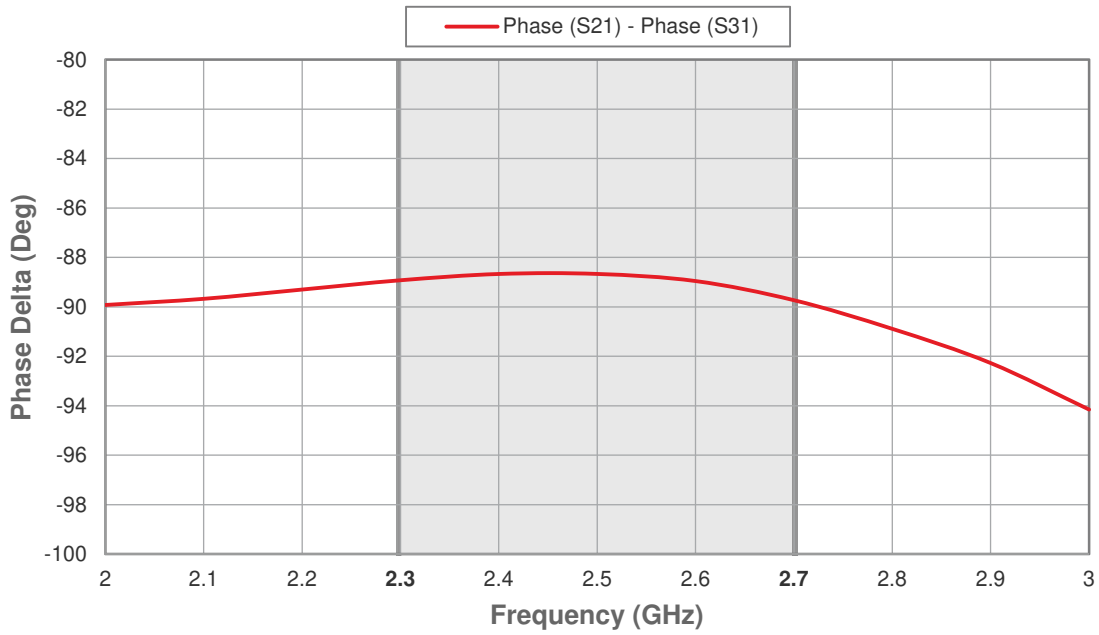
Figure 3 • Relative Phase Shift ( RF_{OUT1}\text{--}RF_{OUT2} )
