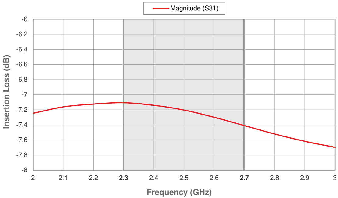
Figure 5 • Insertion Loss ( RF_{IN} - RF_{OUT2} )
