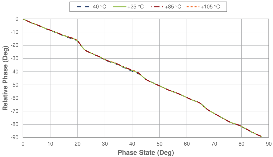
Figure 21 • RF_{OUT2} Relative Phase State Across RF_{OUT2} Phase State vs Temperature, Frequency = 2.5 GHz
