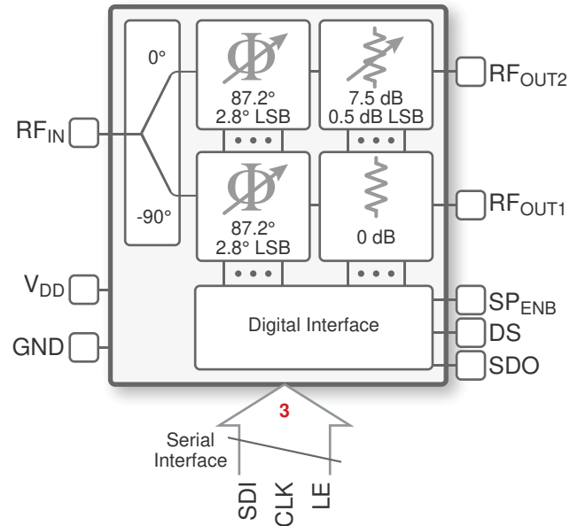
Figure 1 • PE46130 Functional Diagram
