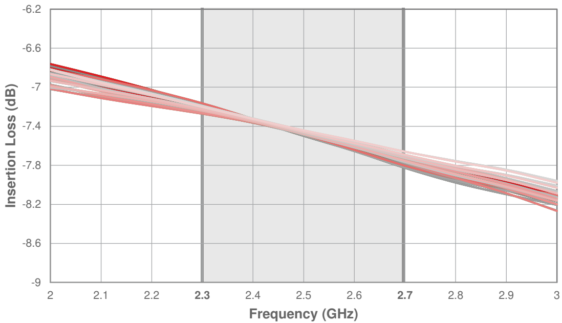
Figure 13 • RF_{OUT1} Insertion Loss Variation Across RF_{OUT2} Phase State
