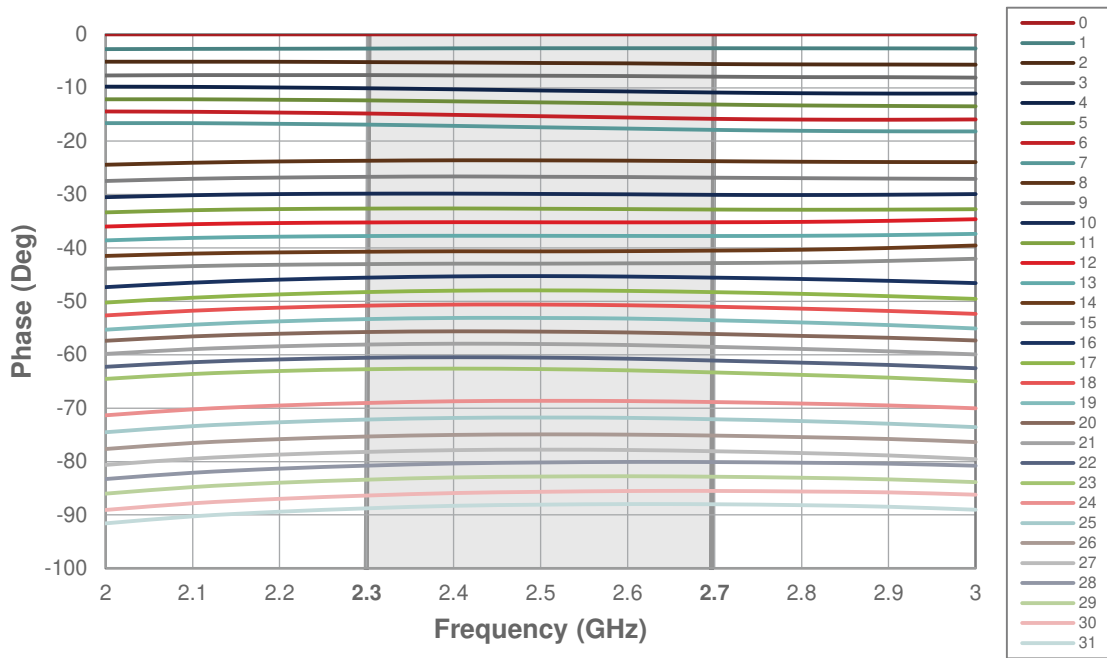
Figure 7 • Relative Phase RF_{IN} - RF_{OUT1} (All RF_{OUT1} Phase States)
