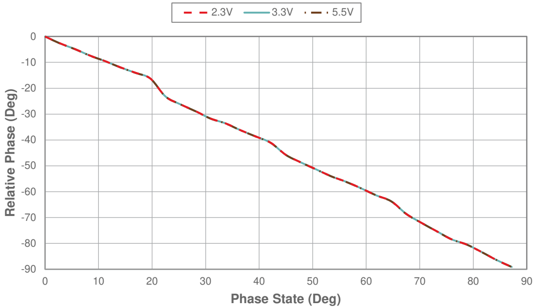
Figure 20 • RF_{OUT2} Relative Phase State Across RF_{OUT2} Phase State vs V_{DD} , Frequency = 2.5 GHz
