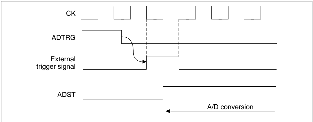
Figure 23.7 External Trigger Input Timing
