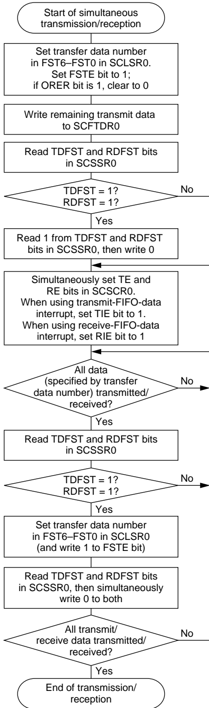
Figure 16.6 Sample SCIF0 Simultaneous Transmission/Reception Flowchart (2)
