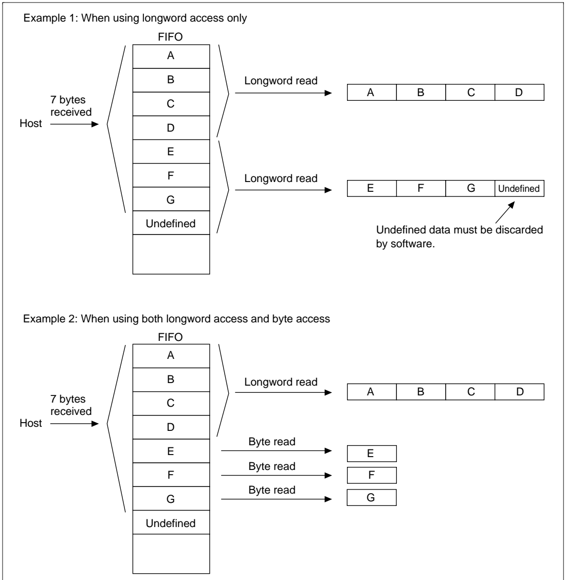
Figure 19.16 Examples of Read Operation when 7 Bytes are Received
