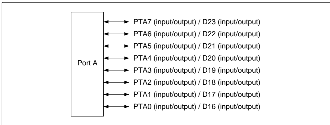
Figure 22.1 Port A
