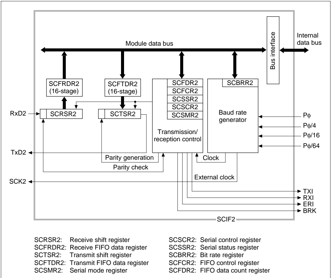
Figure 18.1 Block Diagram of SCIF2
