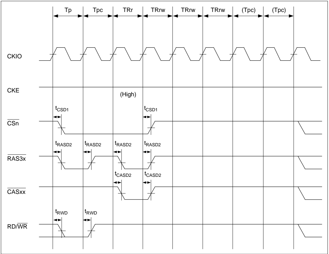
Figure 26.33 Synchronous DRAM Auto-Refresh Timing (TRAS = 1, TPC = 1)
