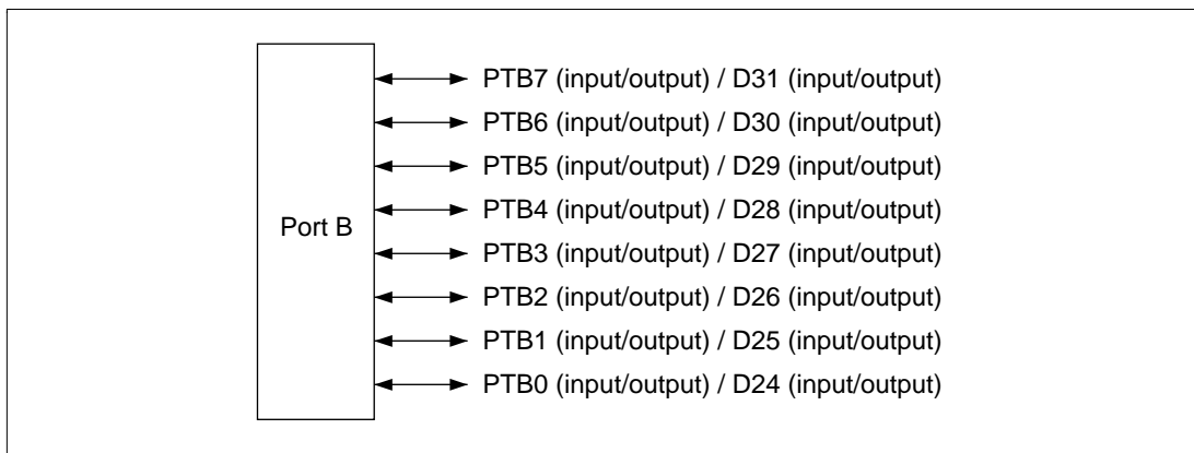
Figure 22.2 Port B
