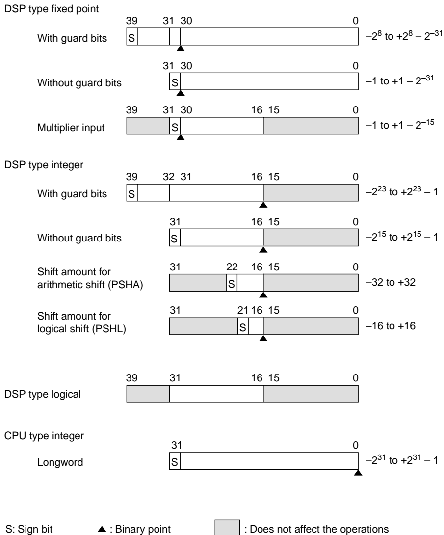
Figure 2.7 Data Format
