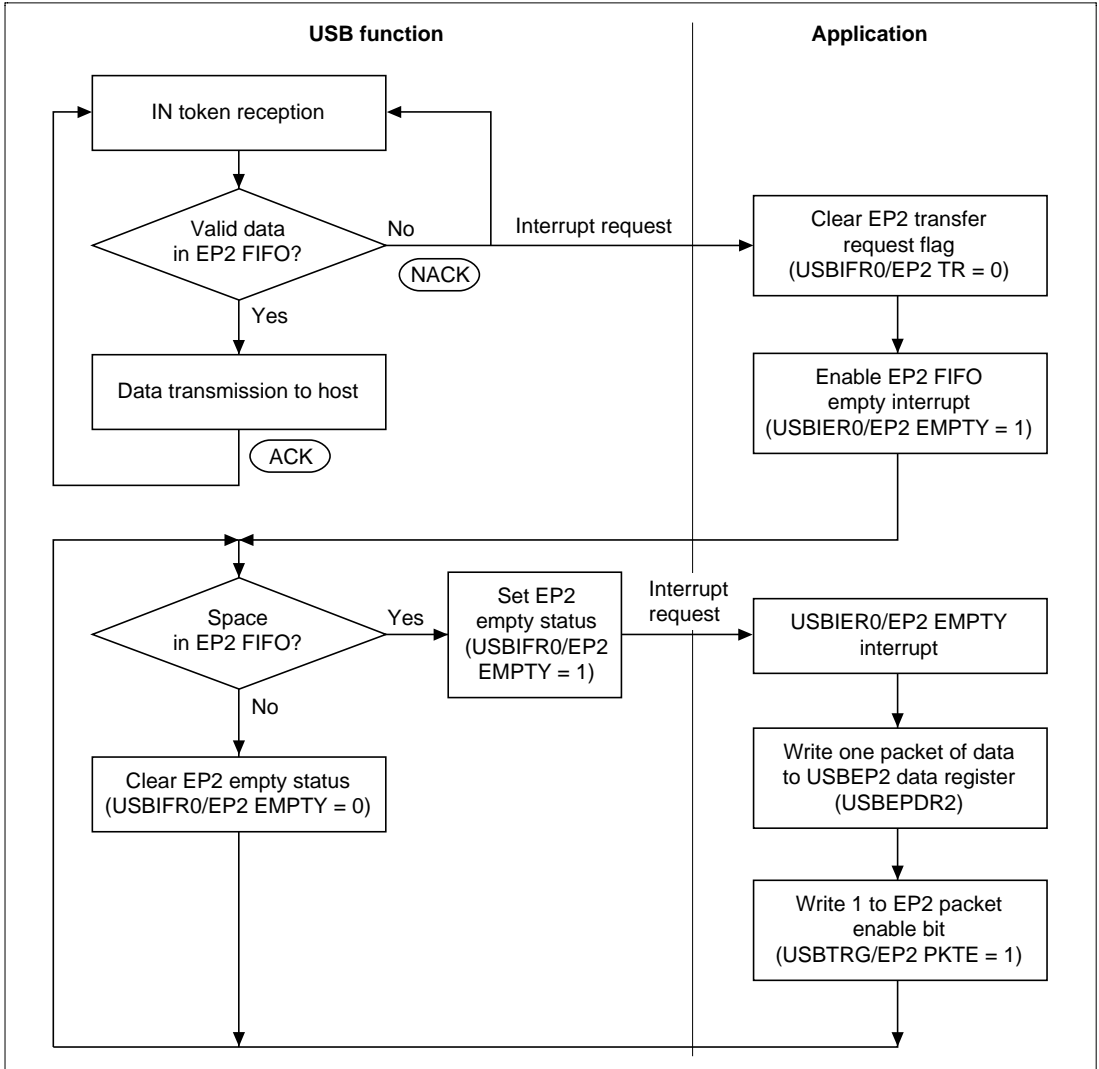
Figure 19.11 EP2 Bulk-In Transfer Operation
