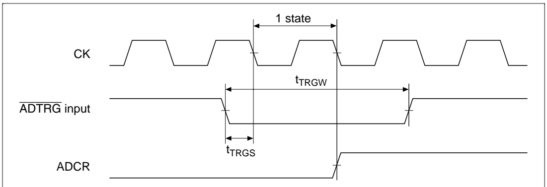
Figure 26.49 External Trigger Input Timing
