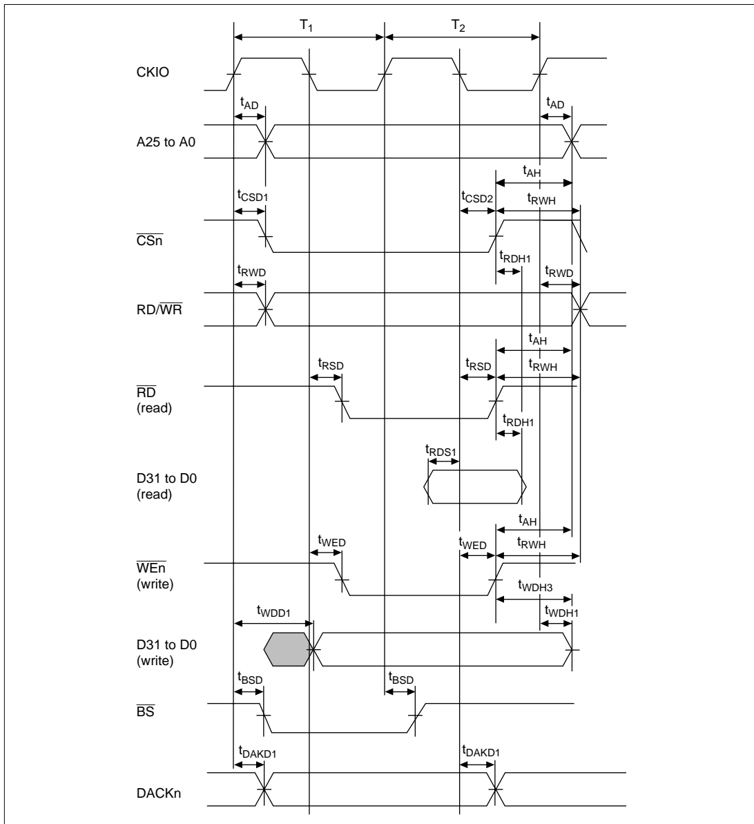
Figure 25.12 Basic Bus Cycle (No Wait)
