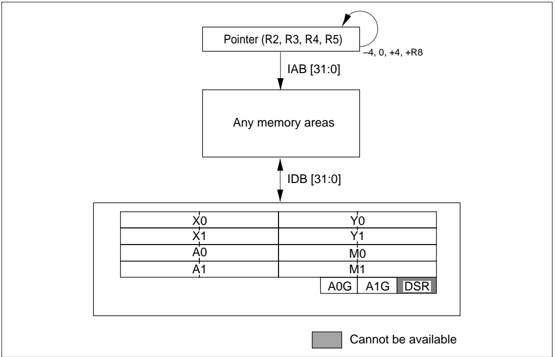
Figure 3.16 Longword of Data-Transfer Operation Flow
