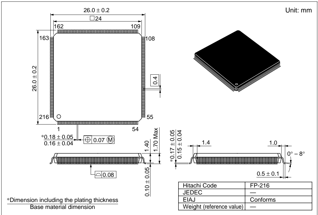
Figure E.1 Package Dimensions (FP-216)
