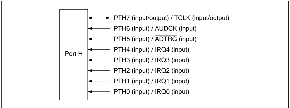
Figure 22.8 Port H
