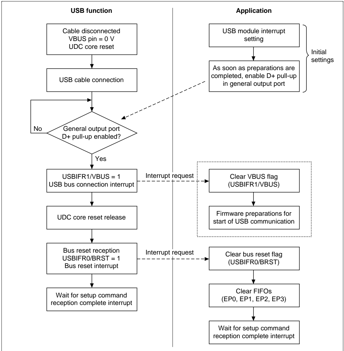
Figure 19.2 Cable Connection Operation
