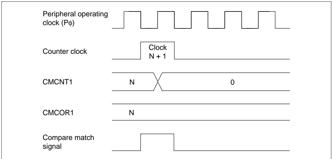
Figure 20.4 Timing of CMF Setting
