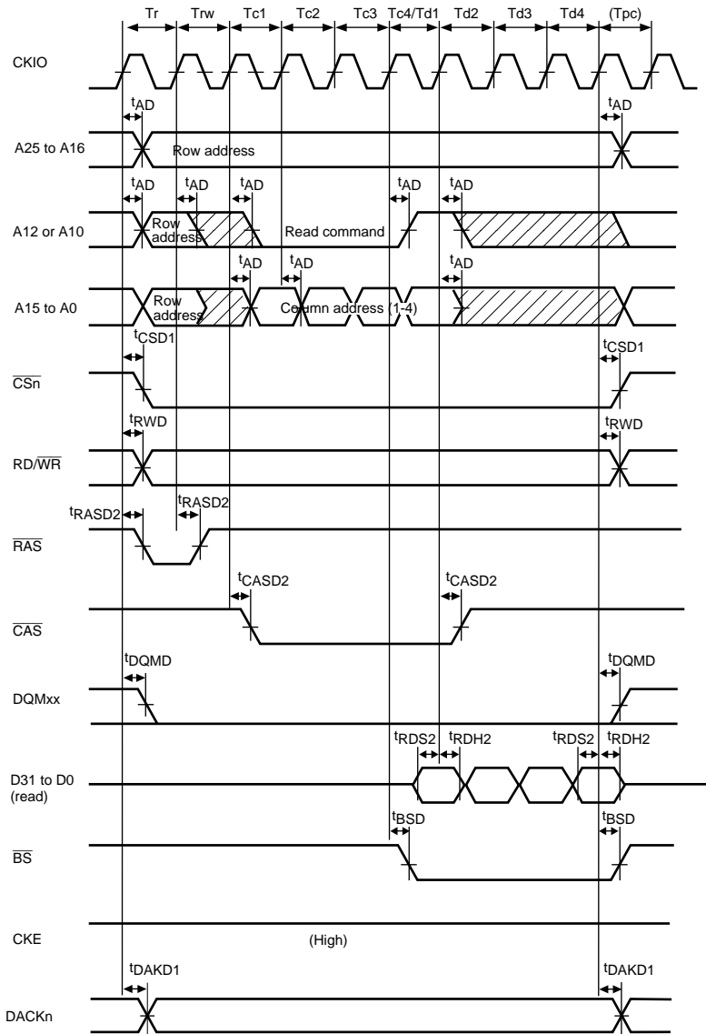
Figure 25.21 Synchronous DRAM Read Bus Cycle (Burst Read (Single Read × 4), RCD = 1, CAS Latency = 3, TPC = 0)
