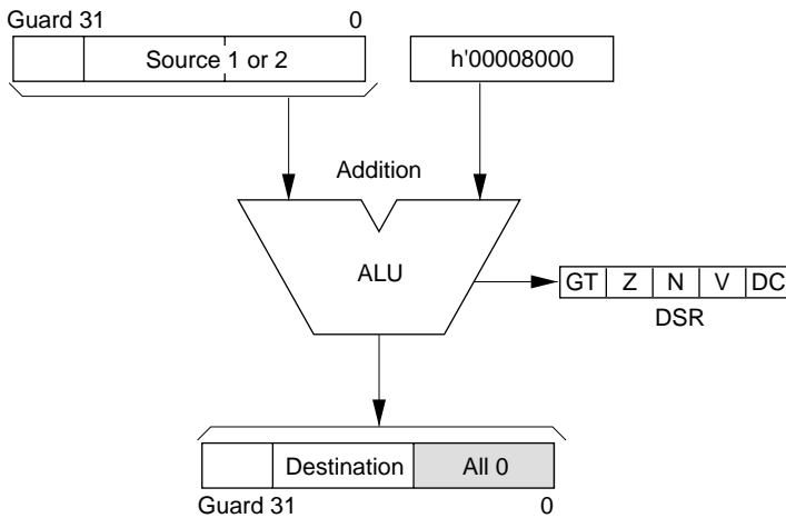
Figure 3.12 Rounding Operation Flow
