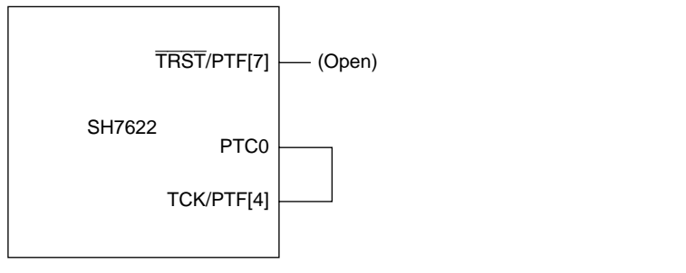
Figure 10.2 Example of Circuit Connections
