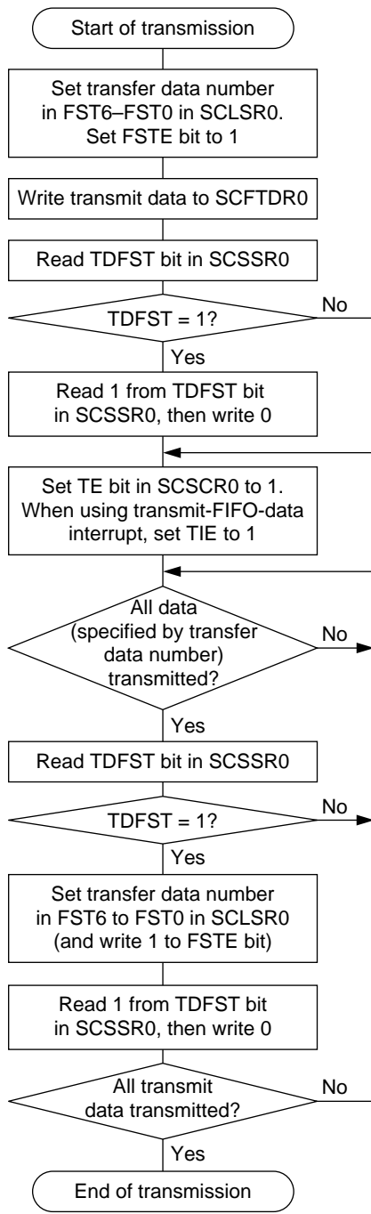
Figure 16.4 Sample SCIF0 Transmission Flowchart (2)
