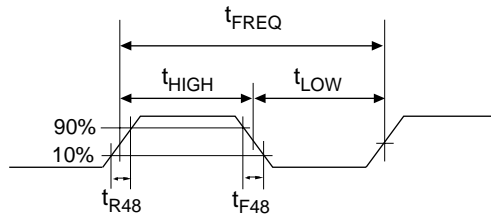
Figure 25.43 USB Clock Timing
