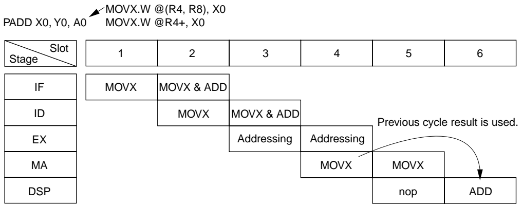
Figure 3.2 Operation Sequence Example
