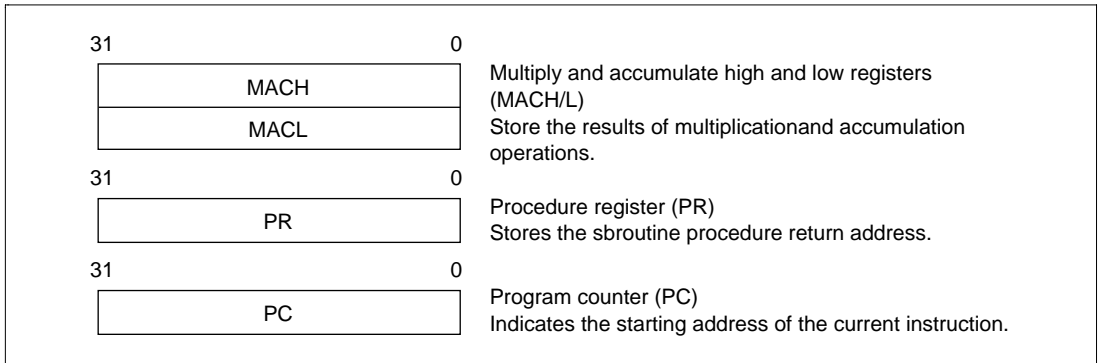
Figure 2.3 System Registers
