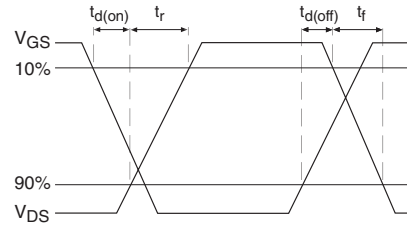
Fig 25b. Switching Time Waveforms
