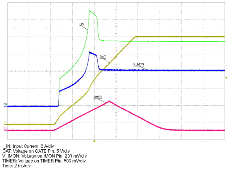
Figure 29. Inrush Mode at Hot-Swap Circuit Insertion
