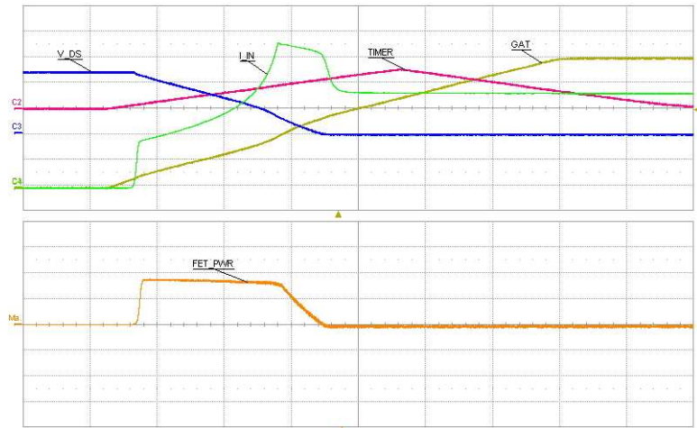
I_IN: Input Current, 2 A/div GAT: Voltage on GATE Pin, 5 V/div V_DS: Drain-to-Source Voltage of M1, 5 V/div TIMER: Voltage on TIMER Pin, 500 mV/div FET_PWR: Power on M1 (product of V_DS and I_IN), 19 W/div Time: 10 ms/div
