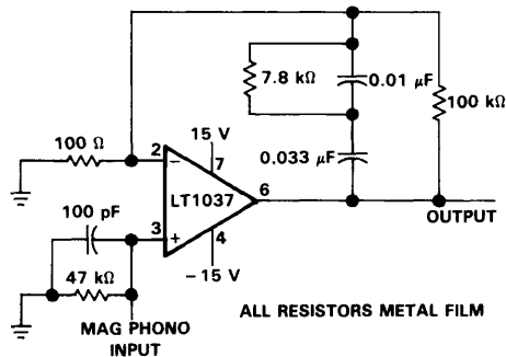
FIGURE 47. PHONO PREAMPLIFIER
