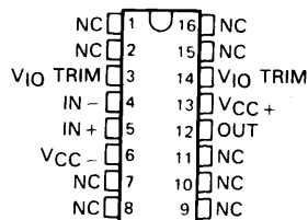
DW SMALL-OUTLINE PACKAGE (TOP VIEW)
